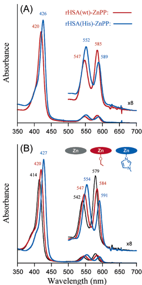
Figure 1. (A) UV-vis absorption spectra of rHSA(wt)-ZnPP and rHSA(His)-ZnPP ( 10 \mu\text{M} ) in potassium phosphate buffered solution (pH 7.0, 10 mM) at 25^\circ\text{C} . (B) UV-vis absorption spectra of ZnPPDME ( 10 \mu\text{M} ) in toluene solution with EtOH (5 vol %) or 1-methylimidazole (5 mM) at 25^\circ\text{C} .
