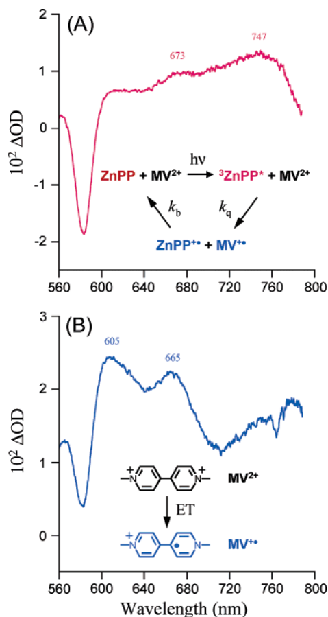
Figure 3. Transient absorption spectra of rHSA(wt)-ZnPP (10 \mu M) with MV ^{2+} (1 mM) in phosphate buffered solution (pH 7.0, 10 mM) after the laser flash photolysis ( \lambda = 532 nm) under argon atmosphere at 25 ^{\circ} C. (A) Spectrum after 100 ns, and (B) spectrum after 200 \mu s.
